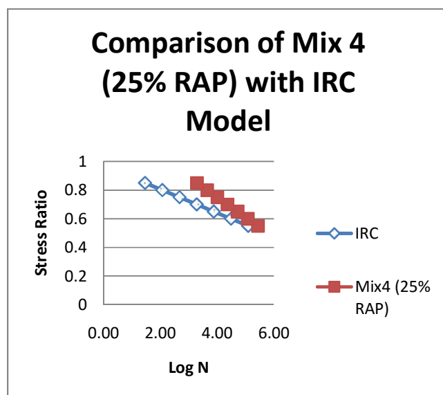
Fig-5.3: Comparison of Mix 4 (25% RAP) with IRC Model
