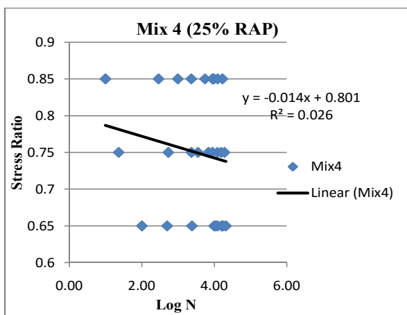
Fig-5.1: Scatter Diagram & Linear Relationship for Mix 4
