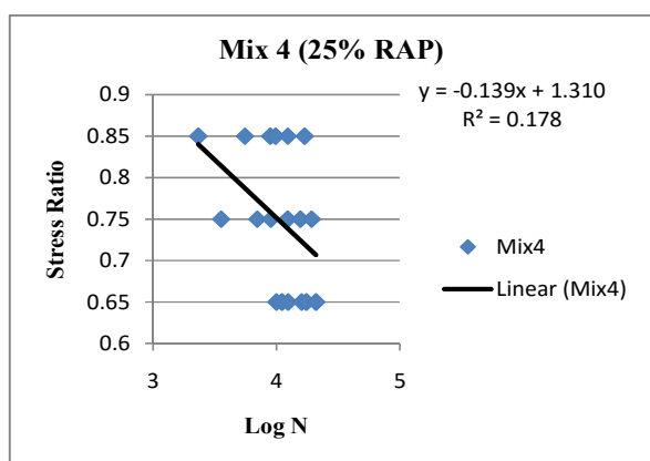
Fig-5.2: Scatter Diagram & Linear Relationship for Mix 4 with Omitted Values
