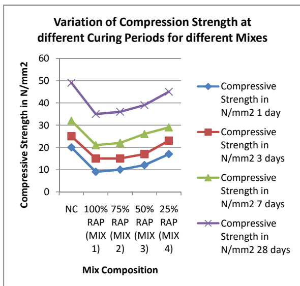
Fig-4.1: Graph showing Compressive Strength Development of Different Mixes
